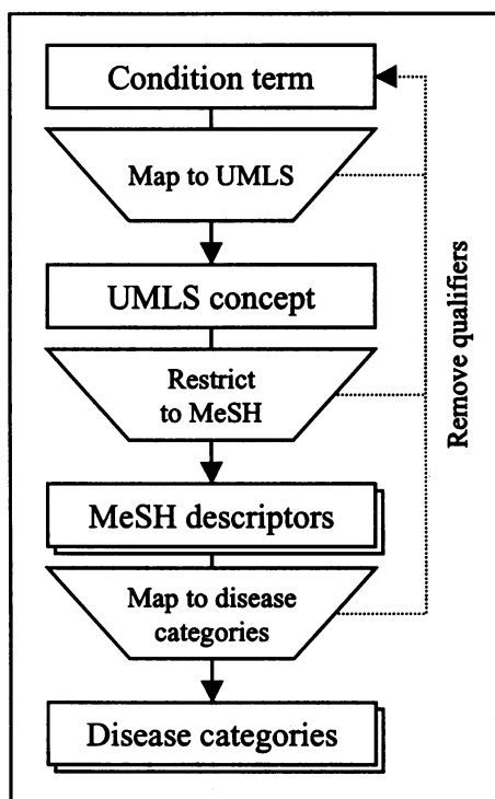
Figure 1 – Classification strategy.
