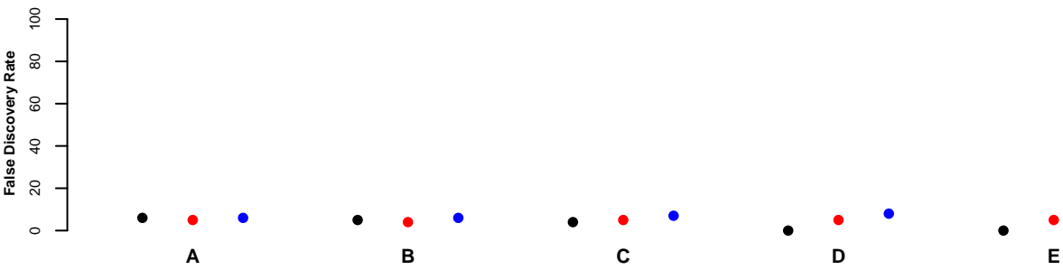
The false discovery rate
