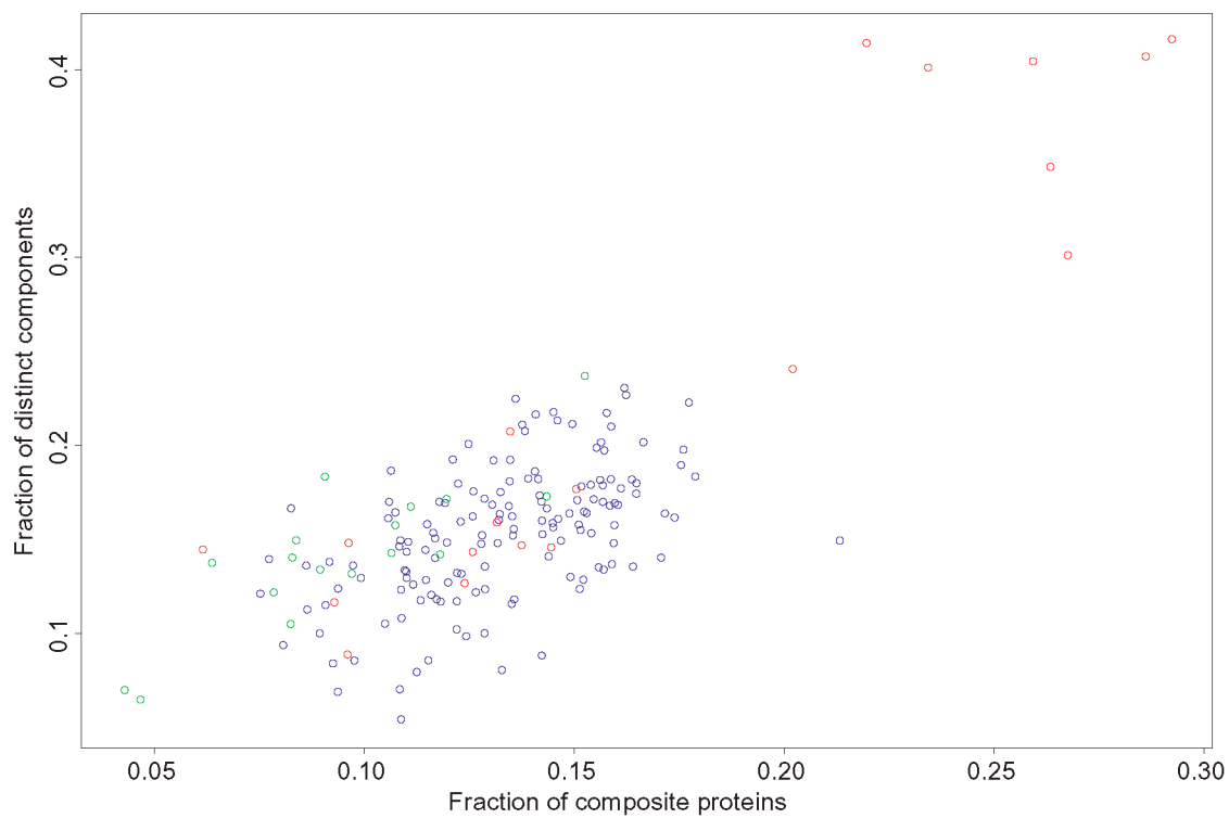
Fraction of distinct components VS fraction of composite proteins
