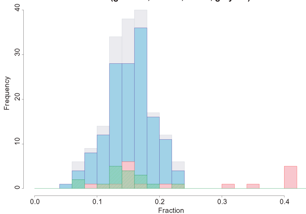
Distribution of fraction of distinct interacting proteins among species (green=A, blue=B, red=E, grey=all)
