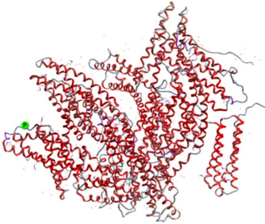
IPI00291175 S290 1tr2 (Vinculin)
