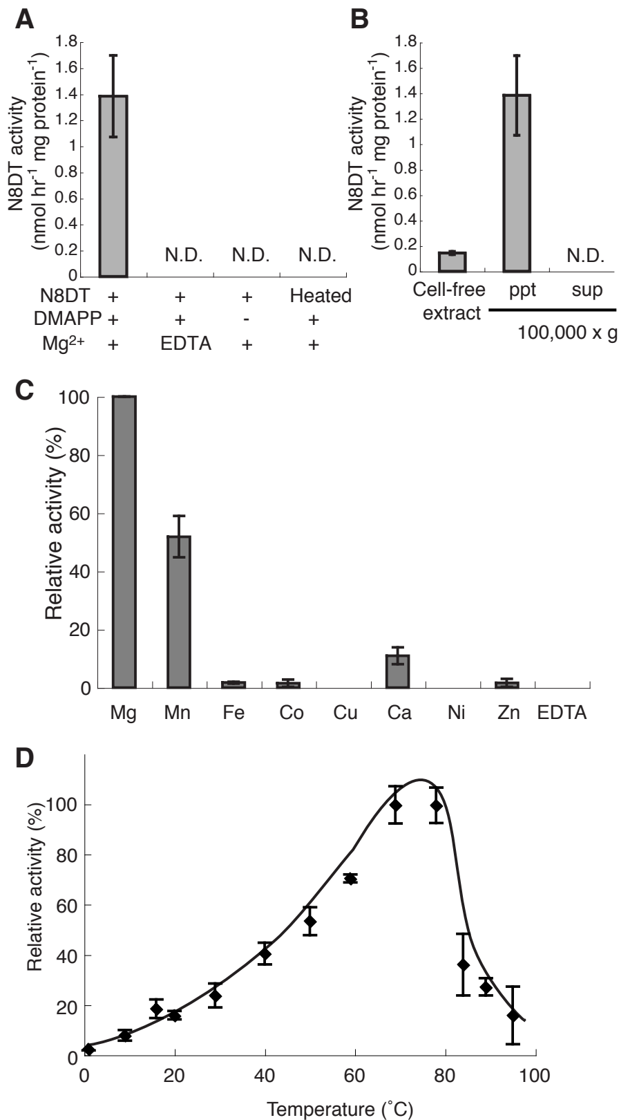
Fig. S1 Enzymatic characterization of recombinant SfN8DT-1 expressed in yeast. (A) Dependency of N8DT activity on Mg 2+ and DMAPP. (B) Separation of N8DT activity in the microsomal fraction from the soluble fraction. (C) Divalent cation requirement. (D) Temperature dependency. N. D., not detected.
