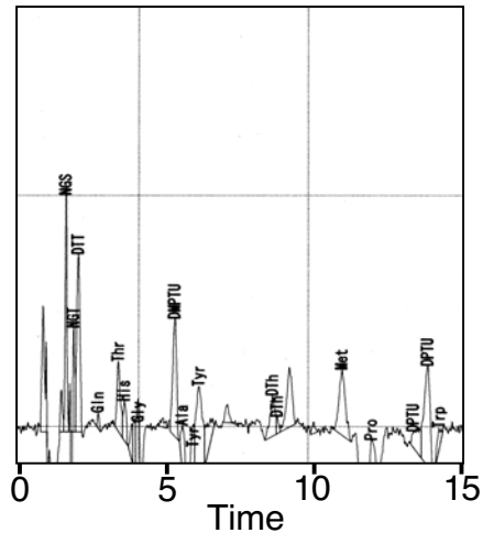
b: Thr31
