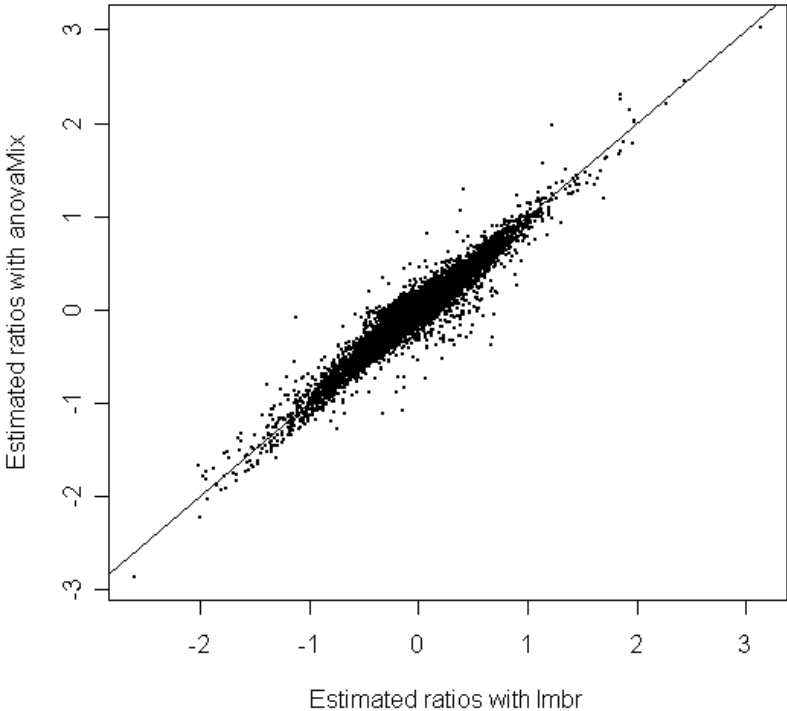
Figure S1: Comparison of corresponding ratios estimated by two linear methods (lmbr and anovaMix) using the loop design. The line indicates the identity between both methods and most of the points are situated near this identity line.
