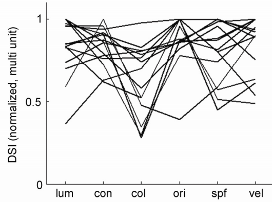
Supplementary Figure 1. Discontinuity sensitivity index of the 15 multi-unit recordings with strong surround suppression ( SI > 0.5 ). The DSIs (lum: luminance; con: contrast; cor: colour; ori: orientation; spf: special frequency; vel: velocity) are normalized by the highest DSI of each cell. Each line represents data from one recording.
