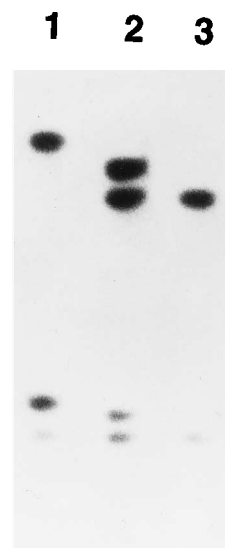
FIG. 2. mecA-ClaI ::Tn554 typing of MRSA clinical isolates from Hospital Pulido Valente. Lane 1, HPV15 ( mecA-ClaI type III::Tn554 type \alpha ); lane 2, HPV12 ( mecA-ClaI type II::Tn554 type J); lane 3, HPV107 ( mecA-ClaI type I::Tn554 type E).
