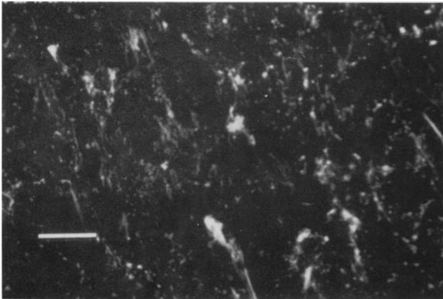
Figure 7. Fluorescent micrograph of F-actin distribution in CEF-populated collagen lattice treated with 2 \mu M cytochalasin D for 15 min. Severe disruption of actin morphology occurred, with the loss of actin bundles. Aggregates of F-actin appear at sites of cell-cell attachment. Bar, 25 \mu m.
