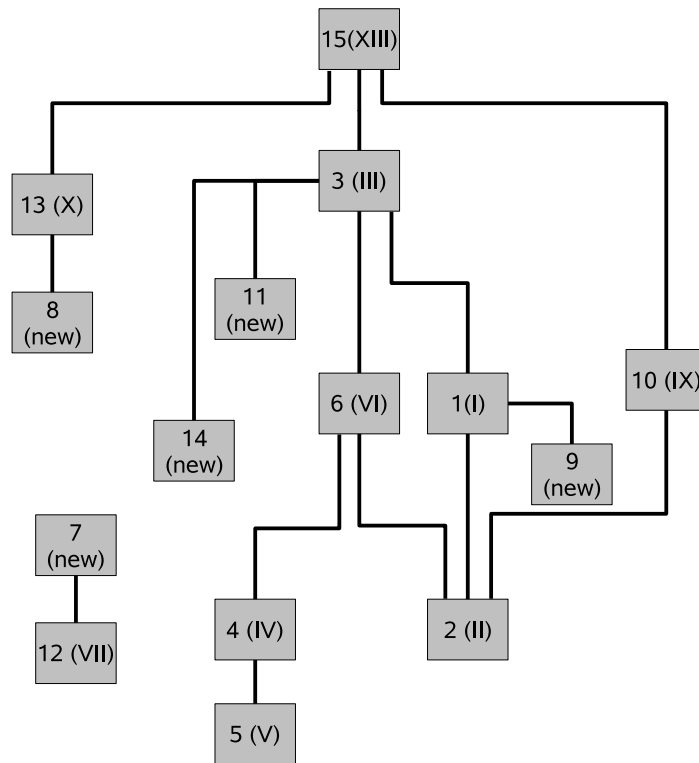
Figure S2: Hierarchy of metabolites for anaerobic conditions. Same as Figure S1, but only water (and no oxygen) has been added to the seeds. As discussed in the text, some clusters are reduced in size. Therefore, some of the small clusters are not included in the figure, whereas others are newly incorporated. It can be seen that the clusters also present in Fig. S1 are ordered in an analogous hierarchy as in the aerobic case.
