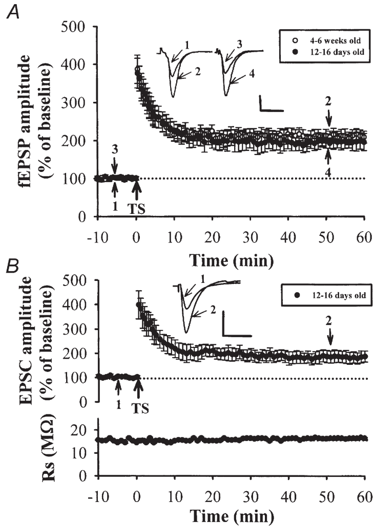
A, summary of experiments showing that tetanic stimulation of mossy fibre produced a robust LTP of fEPSPs in slices obtained from both 4- to 6-week-old (○; n = 12 ) or 12- to 16-day-old mice (●; n = 6 ). B, summary of experiments ( n = 5 ) showing that tetanic stimulation of mossy fibre elicited a robust LTP of whole-cell EPSCs at -70 mV holding potential. Series resistances ( R_s ) were continuously monitored throughout the experiments.
