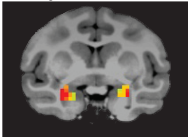
Monkey B
