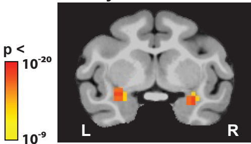
Monkey B
