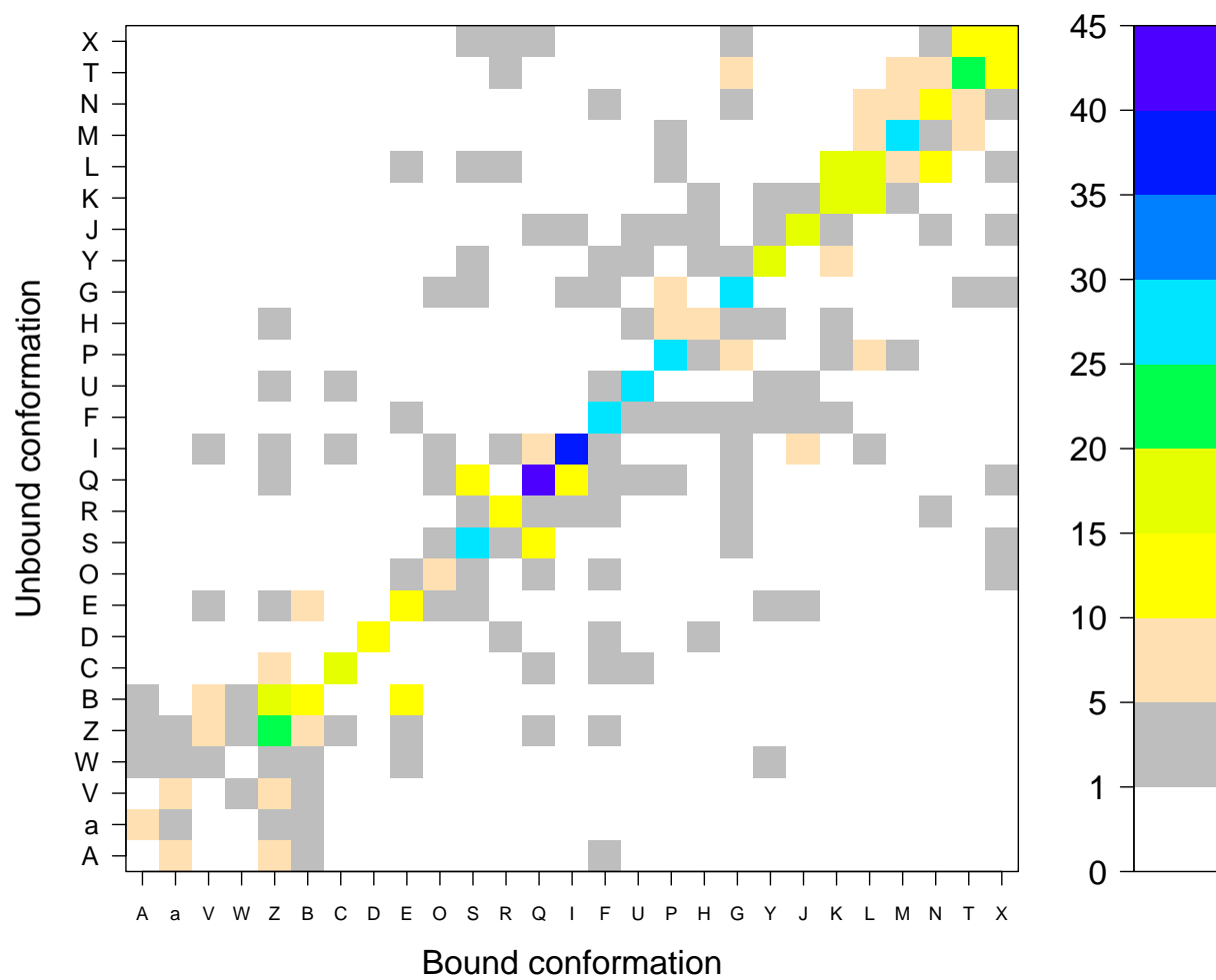
Figure 1: Number of structural letter substitutions corresponding to local rmsd greater than 0.2\text{\AA} , in the interface region of the complex set. The total number of structural letter pairs is 1309.
