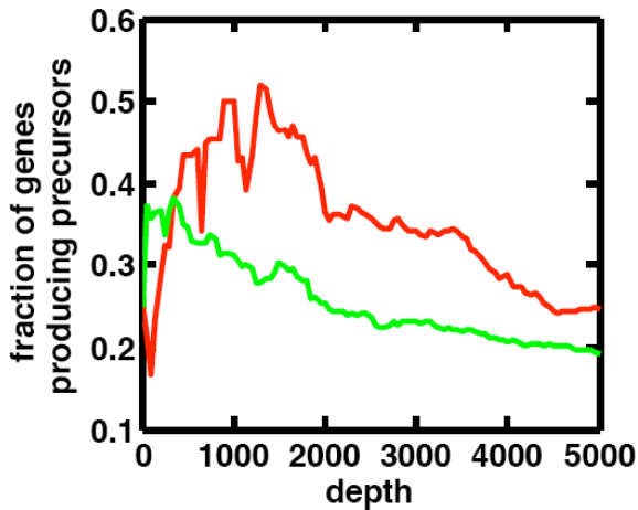
Figure S8. Fraction of genes producing precursors
