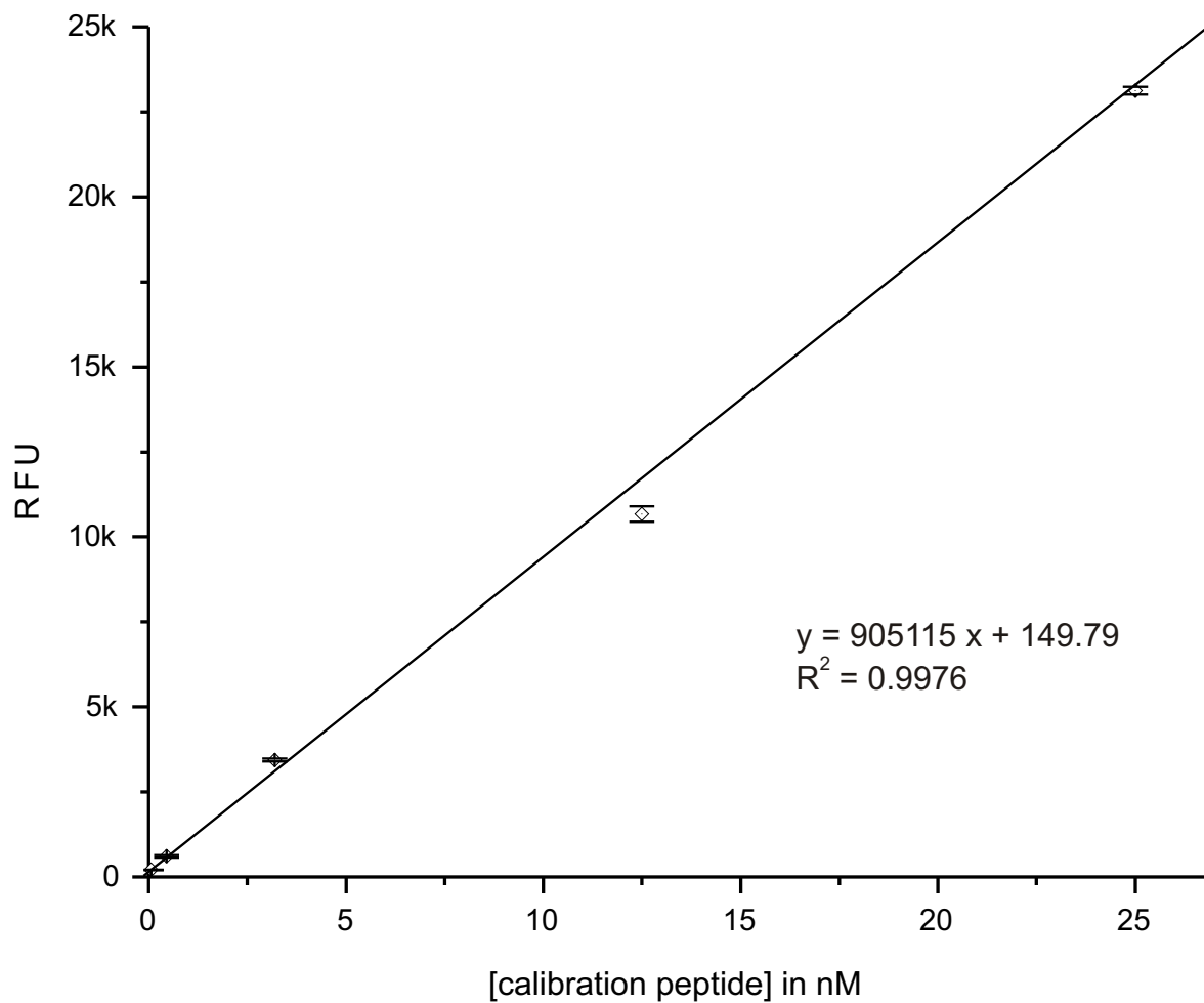
Figure S3: Standard curve of the fluorescence signal of the unquenched calibration peptide, which is structurally identical to the FITC-containing cleavage product resulting from BoNT/A hydrolysis of SNAPtide by BoNT/A; y in RFU; x in nM; R is the correlation coefficient
