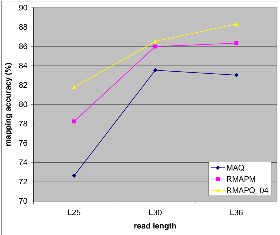
Supplementary figure 1: Accuracy comparison with MAQ: mapping accuracies of MAQ, RMAPM and RMAPQ. Three different read lengths were used {25bp, 30bp, 36bp}. Default parameter setting is used for MAQ. Two mismatches are allowed for RMAPM and RMAPQ, and quality score cutoff for RMAPQ is 4. Mapping accuracy = (coverage + selectivity)/2 (see main text).
