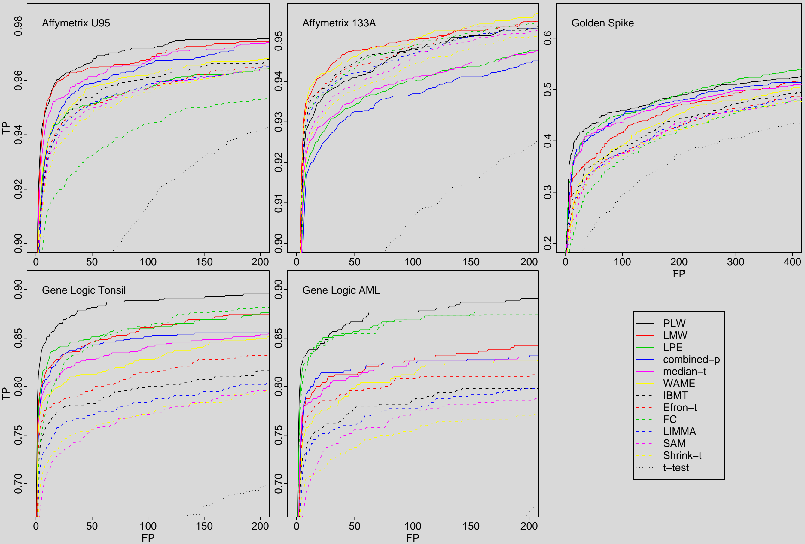
Figure S1: ROC curves based on RMA pre-processed data
