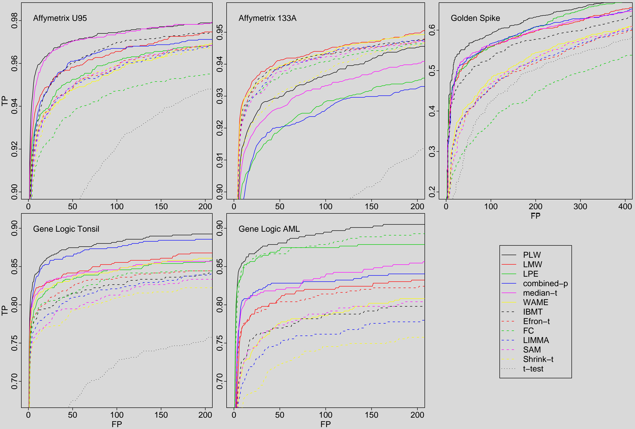
Figure S2: ROC curves based on GCRMA pre-processed data
