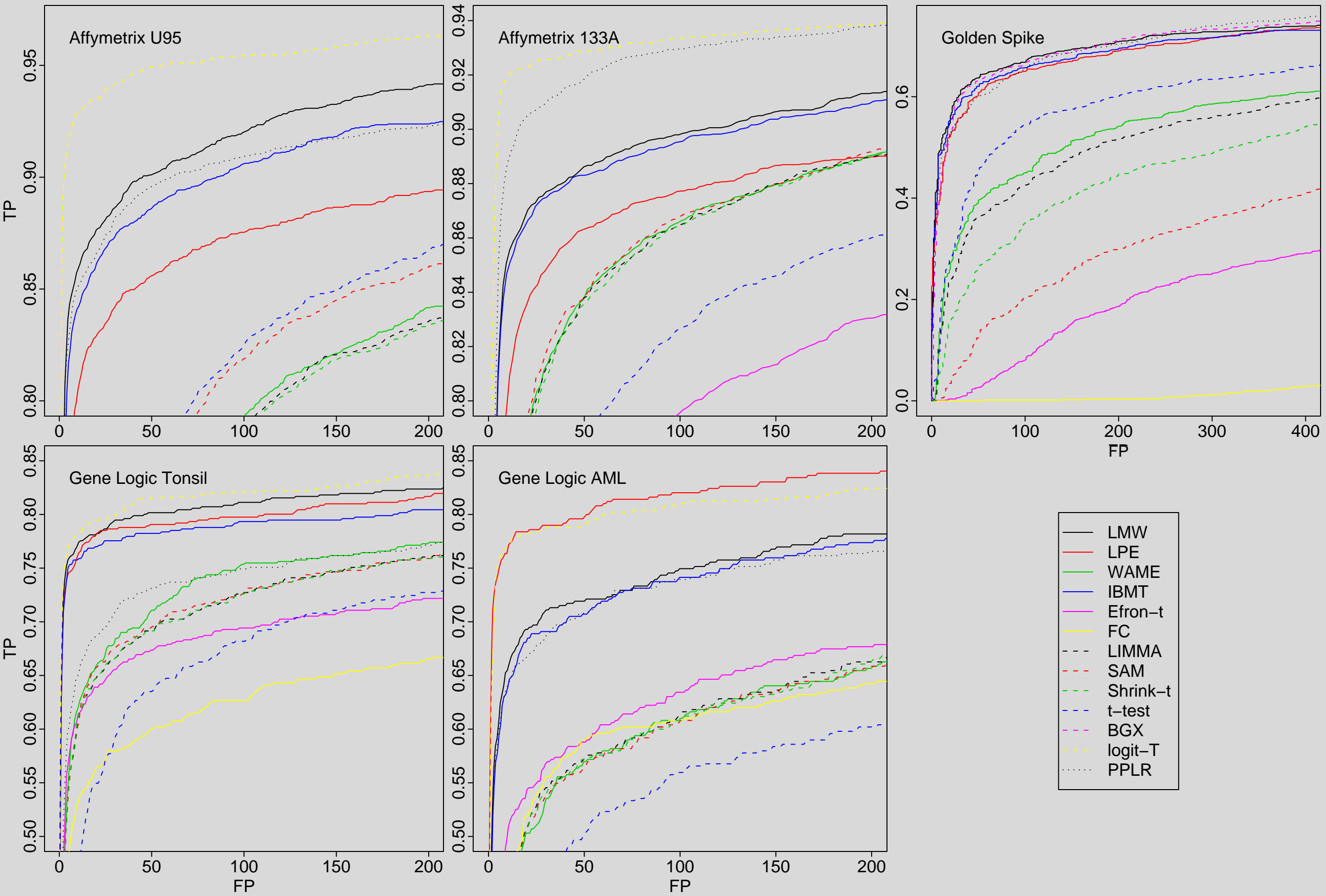
Figure S3: ROC curves based on MAS5 pre-processed data, together with ROC curves for PPLR, BGX, and logit-t Note the range of y axis, line colors, and line types differs from Figures S1 and S2
