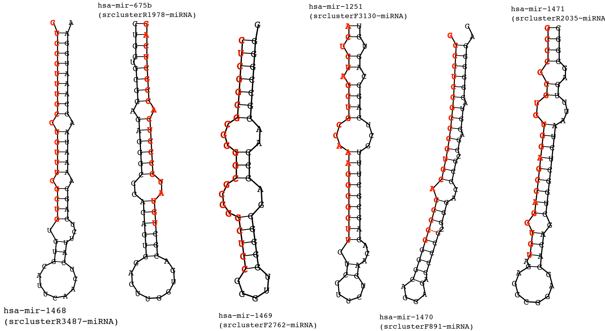
Figure S14. Predicted secondary structures of the novel miRNAs
