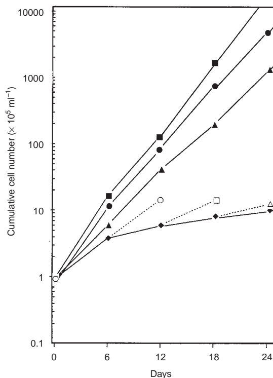
Figure 3 Proliferation of EBC-1 cells in long-term culture with Dex and vesnarinone. Cells were cultured without ( \blacksquare ) or with 2 \times 10^{-8} M Dex ( \bullet ), 10 \mu\text{g ml}^{-1} vesnarinone ( \blacktriangle ), or 2 \times 10^{-8} M Dex plus 10 \mu\text{g ml}^{-1} of vesnarinone ( \blacklozenge ). Open symbols, cells were washed and then cultured without drugs. Cells were treated with Dex plus vesnarinone for 6 ( \circ ), 12 ( \square ) and 18 ( \triangle ) days, and then washed and reincubated without drugs for further 6 days. Data are means of three separate experiments
