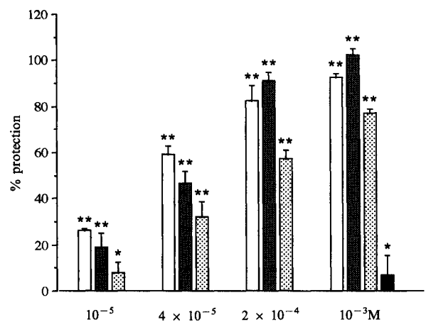
FIG. 4. Protection of HUVEC from MPO/ \text{H}_2\text{O}_2/\text{Cl}^- stress. Comparison of ceftazidime (CAZ) with methionine, histidine and dabco. ^{51}\text{Cr} labelled HUVEC were preincubated with MPO ( 5\ \mu\text{g} ) and variable concentrations of the protectors for 2 h at 37^\circ\text{C} : \square , CAZ; \blacksquare , methionine; \square , histidine; \blacksquare , dabco. \text{H}_2\text{O}_2 ( 10^{-4}\text{M} ) was added to initiate stress and the % protection was calculated after 2 h. The results are expressed as arithmetic mean \pm S.D. of three experiments performed in triplicate. *No statistical difference ( p > 0.05 ) and **statistical difference ( p < 0.05 ) vs. stress without protector when analysed with the two-tailed Student's t -test.
