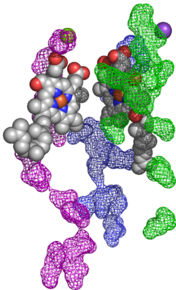
Figure S14. The three proposed proton transfer channels in COI. Channels are expressed by the electron density of amino acids assembling each channel. Channel identification is as follows: channel D (blue), channel H (green), and channel K (magenta).
