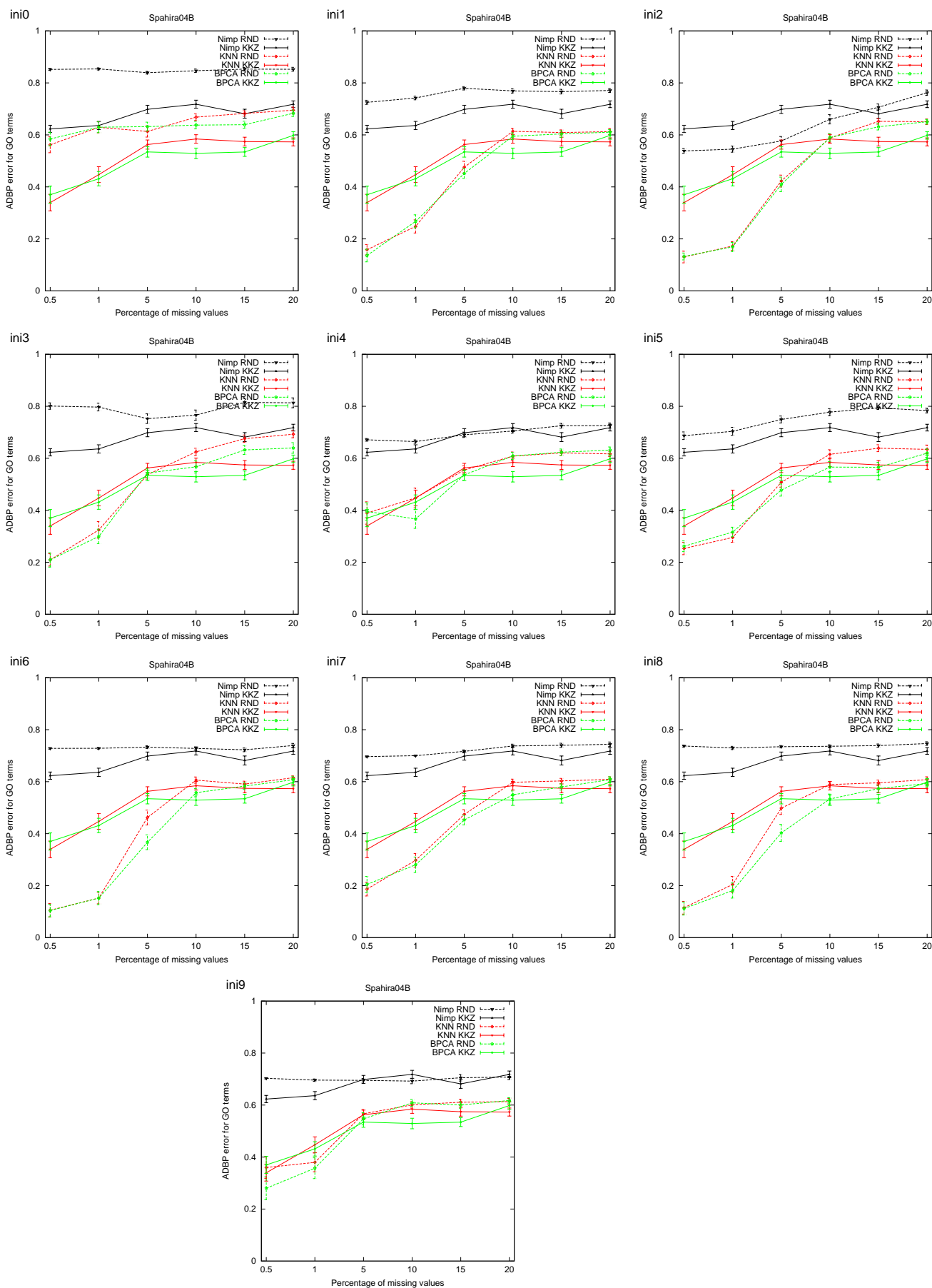
Figure 1: Agreement with the original GO terms when the k -means clustering was initialized from 10 random starting points ( k = 5 ). The solid lines indicate the results from the deterministic KZZ initialization (see Fig. 4), while the dashed lines are the results from the particular random initialization (10 different starting points). The error bars represent the standard error of mean (SEM) values over the 30 replicate missing datasets.
