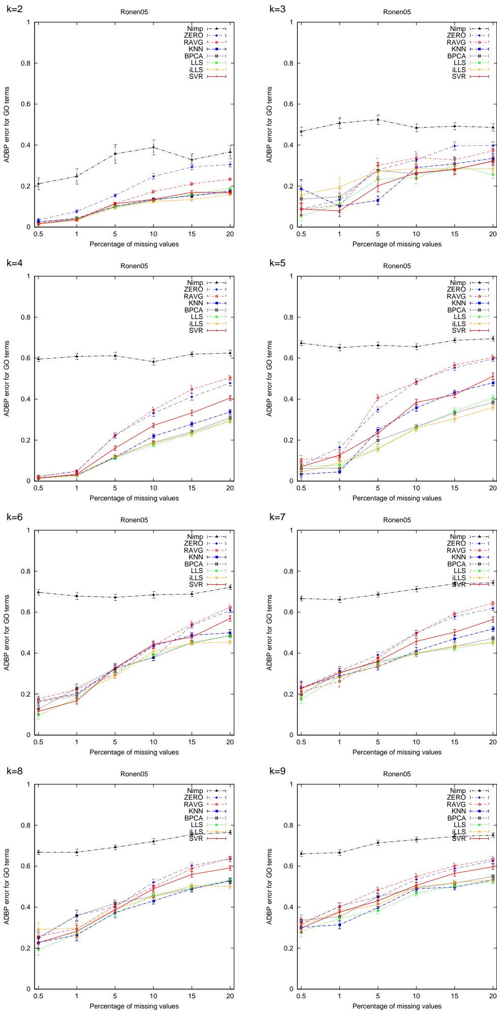
Figure 1: Capability of the k -means algorithm to identify the original GO terms of the clusters in the Ronen05 dataset with or without imputation. The results are presented as the average distance between partitions (ADBP) of genes and the error bars are the standard error of mean (SEM) values over the 30 replicate missing datasets.
