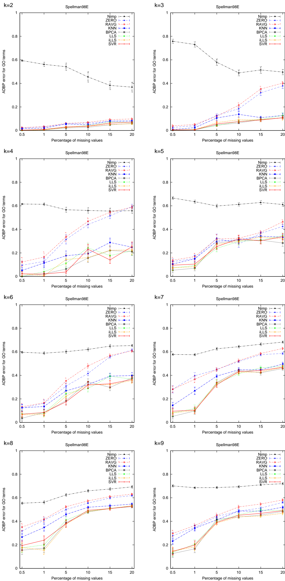
Figure 8: Capability of the k -means algorithm to identify the original GO terms of the clusters in the Spellman98E dataset with or without imputation. The results are presented as the average distance between partitions (ADBP) of genes and the error bars are the standard error of mean (SEM) values over the 30 replicate missing datasets.
