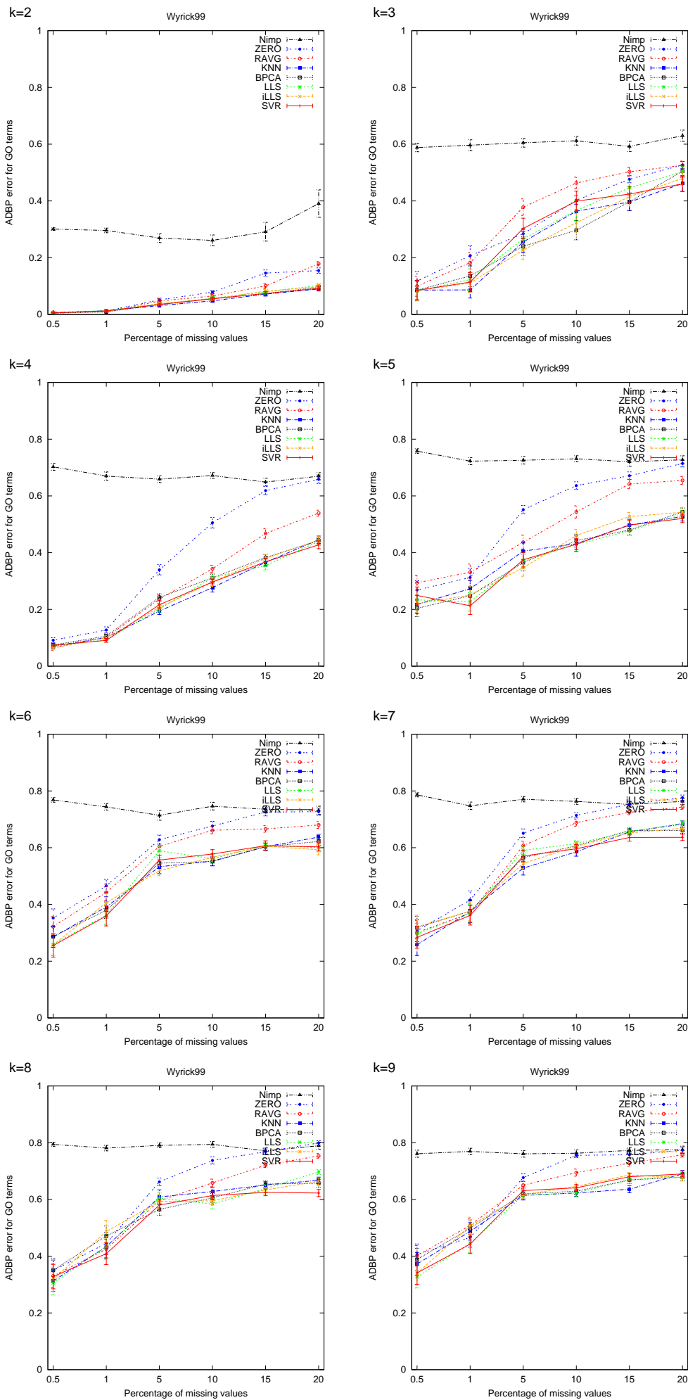
Figure 7: Capability of the k -means algorithm to identify the original GO terms of the clusters in the Wyrick99 dataset with or without imputation. The results are presented as the average distance between partitions (ADBP) of genes and the error bars are the standard error of mean (SEM) values over the 30 replicate missing datasets.
