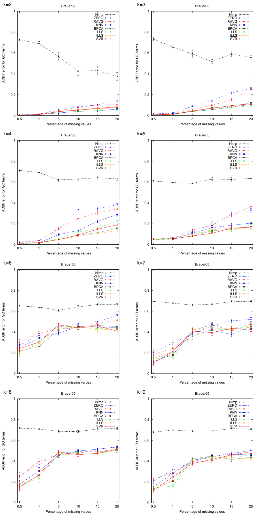
Figure 2: Capability of the k -means algorithm to identify the original GO terms of the clusters in the Brauer05 dataset with or without imputation. The results are presented as the average distance between partitions (ADBP) of genes and the error bars are the standard error of mean (SEM) values over the 30 replicate missing datasets.
