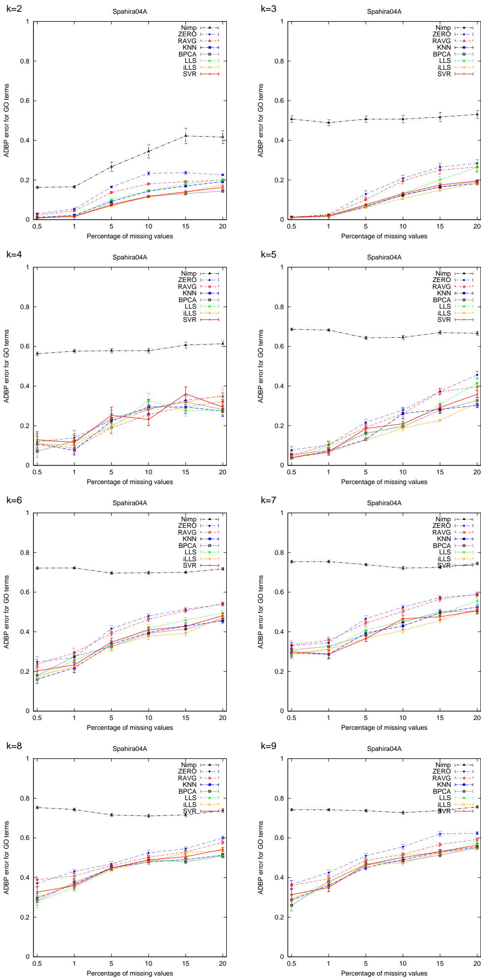
Figure 3: Capability of the k -means algorithm to identify the original GO terms of the clusters in the Spahira04A dataset with or without imputation. The results are presented as the average distance between partitions (ADBP) of genes and the error bars are the standard error of mean (SEM) values over the 30 replicate missing datasets.
