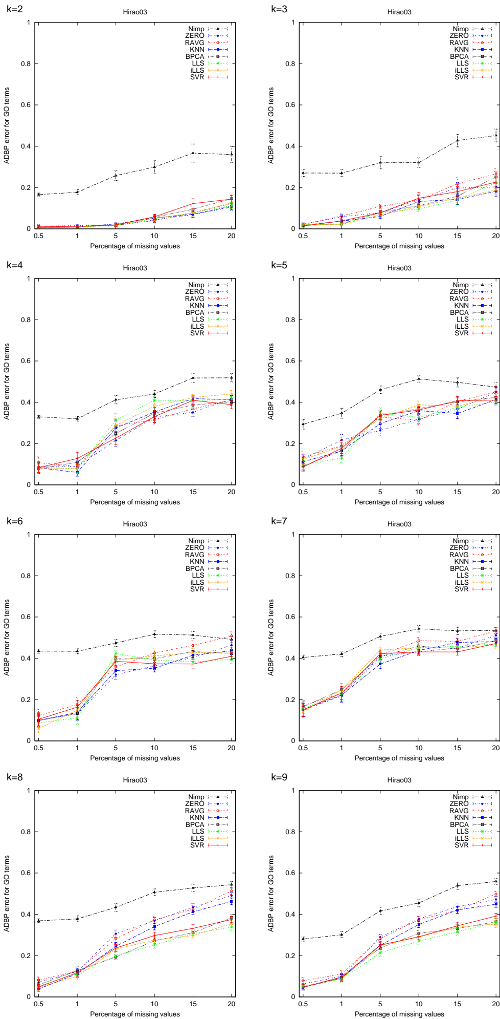
Figure 5: Capability of the k -means algorithm to identify the original GO terms of the clusters in the Hirao03 dataset with or without imputation. The results are presented as the average distance between partitions (ADBP) of genes and the error bars are the standard error of mean (SEM) values over the 30 replicate missing datasets.
