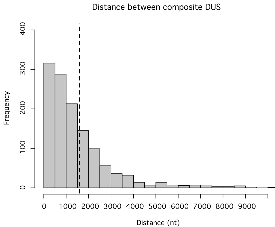
Additional Figure A1 – Distribution of the distance between contiguous composite DUS in the Neisseria meningitidis Z2491 genome.
