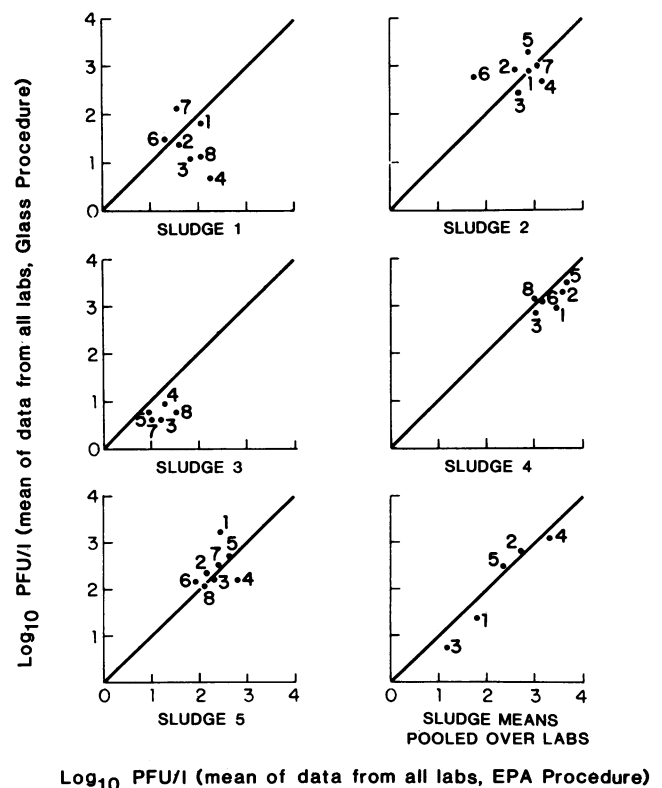
FIG. 2. Reference laboratory quality assurance data for sludges.
