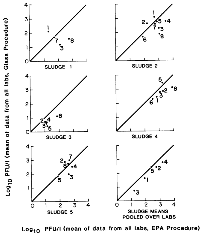
FIG. 1. Round robin comparison data for sludges.
