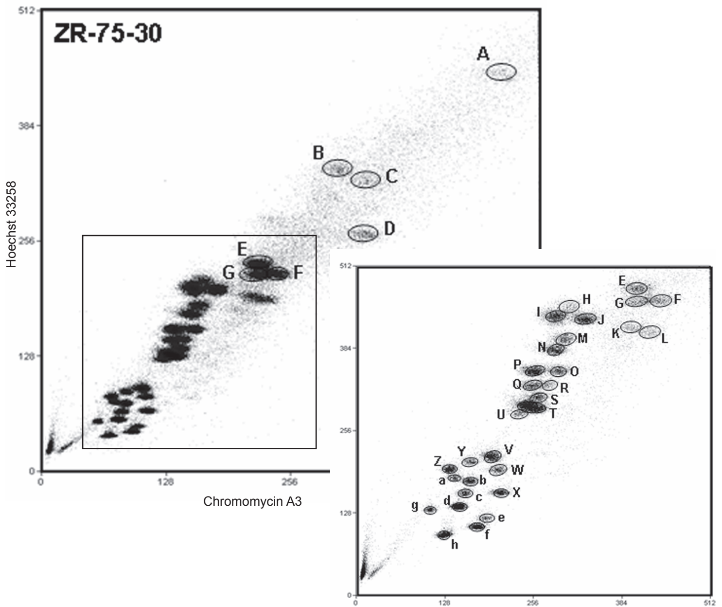
Supplementary Figure 2 Flow karyotype of chromosomes from the breast cancer cell line ZR-75-30. Axes as in figure 1. The 'peaks' are designated A to h. In the inset the gain has been increased to show the smaller peaks more clearly.
