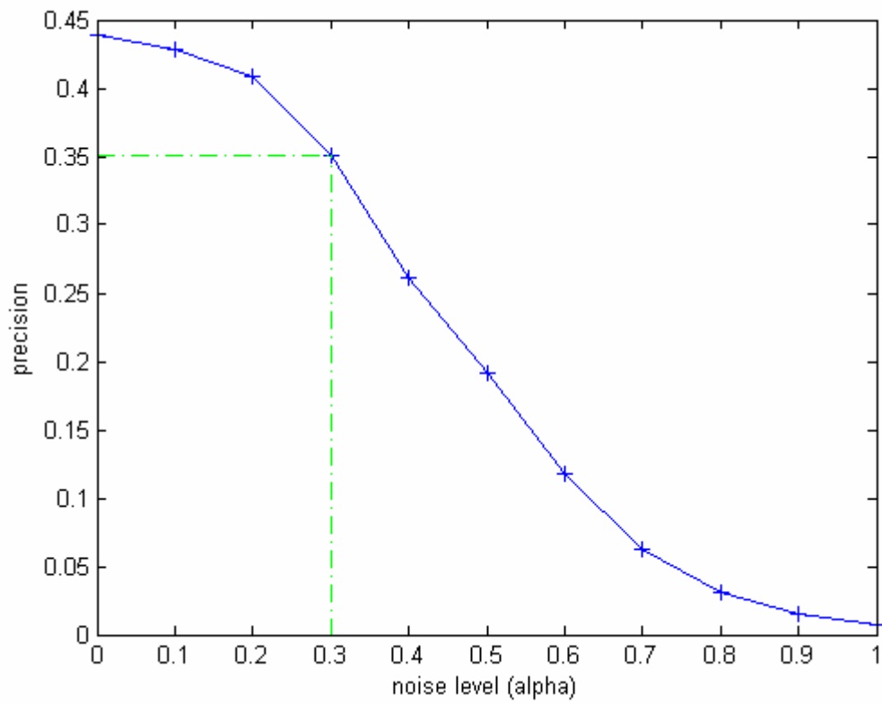
Supplementary Figure S1. This figure shows how the precision varies with noise level (the coefficient alpha).
