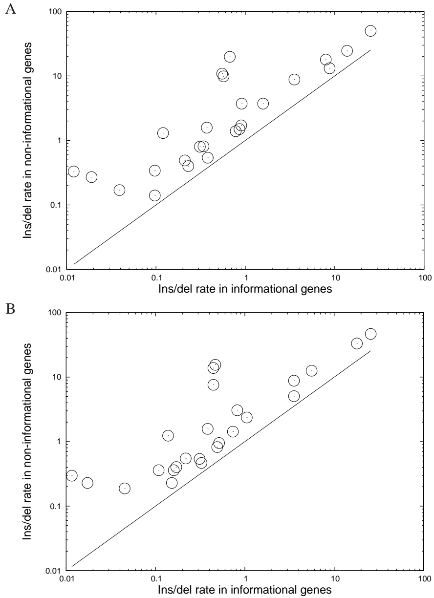
Figure S.1: Different ins/del rates between informational genes and non-informational genes. A, estimation was based on the select-genes trees; B, estimation was based on the common-genes trees. Only constant rates with no rate variation are shown, and the y = x line is also shown.
