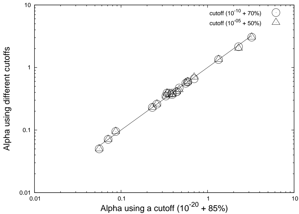
Figure S.5: \alpha value after informational genes were removed using different cutoffs on e-value and match length in identifying informative genes. Estimation was based on the select-genes trees. Maximum likelihood estimation was conducted by only using the best supported phylogeny of each group to reduce computational burden.
