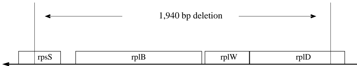
Figure S.3: The deletion of ribosomal proteins in Streptococcus mutans UA159 (GenBank accession: AE014133).
