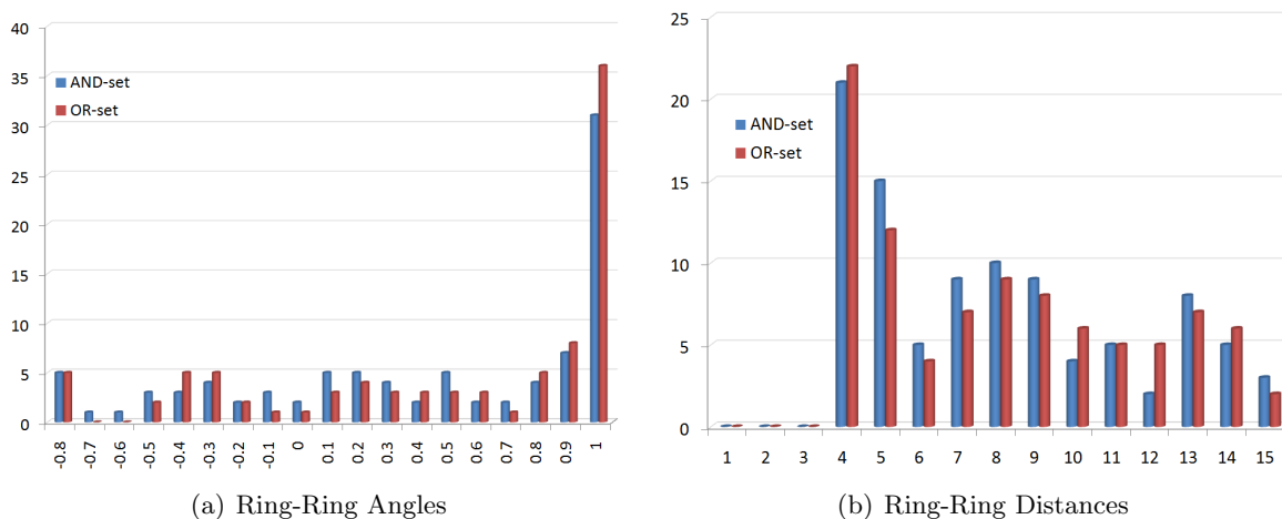
Figure S1: Distribution of ring-ring angles and distances. (a) A histogram of angles between the ring planes of consecutive protein interacting nucleotides. The X-axis is the cosine of the angle. The Y-axis is the frequency of occurrence in the AND-set and OR-set datasets of protein-RNA complexes. (b) An histogram of distances between the ring planes of consecutive protein interacting nucleotides. The X-axis is the distance (in Å). The Y-axis is the frequency of occurrence in the two datasets.
