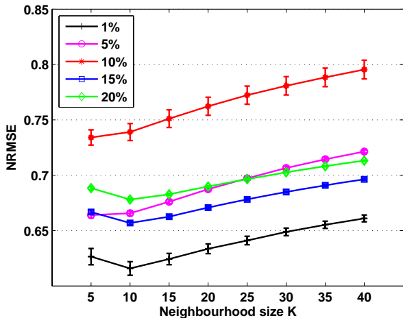
Histone
