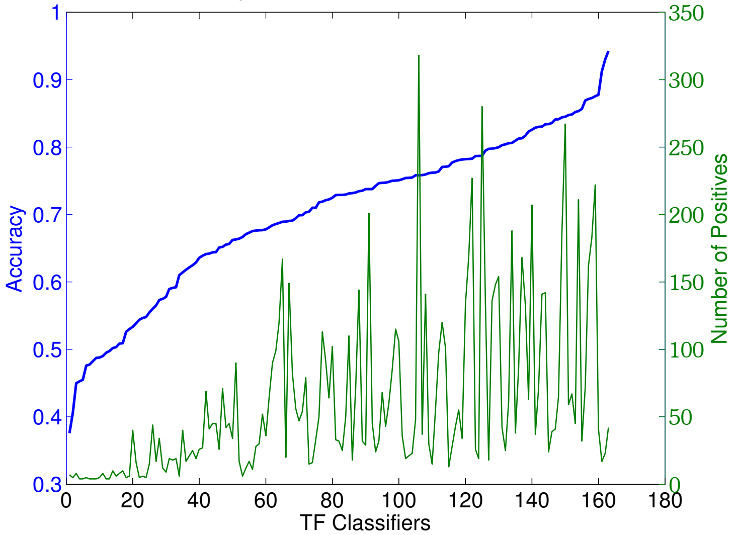
Accuracy and Positives in TF Classifiers
