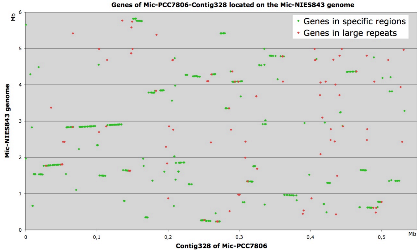
Additional file 1: Representation of the location of the genes of Mic-PCC7806 contig328 on the genome of Mic-NIES843. Two proteins are considered to be identical if they share at least 40% similarity on their total length. Large repeats are defined as DNA regions containing more than 1000 bases and a similarity threshold >90%. See the Methods section for the strain identifiers.
