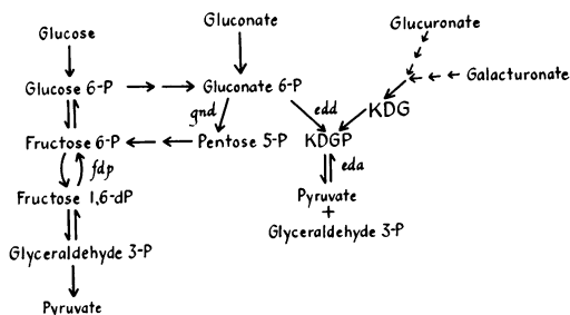
FIG. 1. Pathways of gluconate metabolism. Gene abbreviations are: gnd , gluconate 6-phosphate dehydrogenase; edd , gluconate 6-phosphate dehydrase; eda , KDGP aldolase; and fdp , fructose diphosphatase. KDG is 2-keto-3-deoxygluconate, and KDGP is 2-keto-3-deoxygluconate 6-phosphate.
