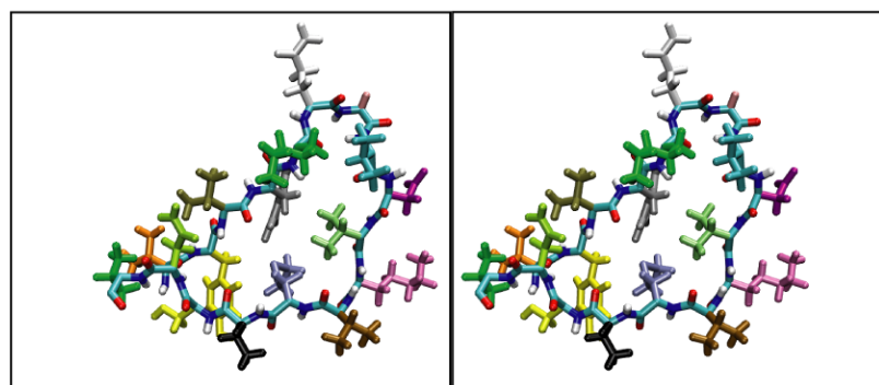
Figure 1: : Stereo views of the initial structure of simulation sets: F_{GOF1} , F_{WT1} , F_{LOF1} . (see Table 2)
