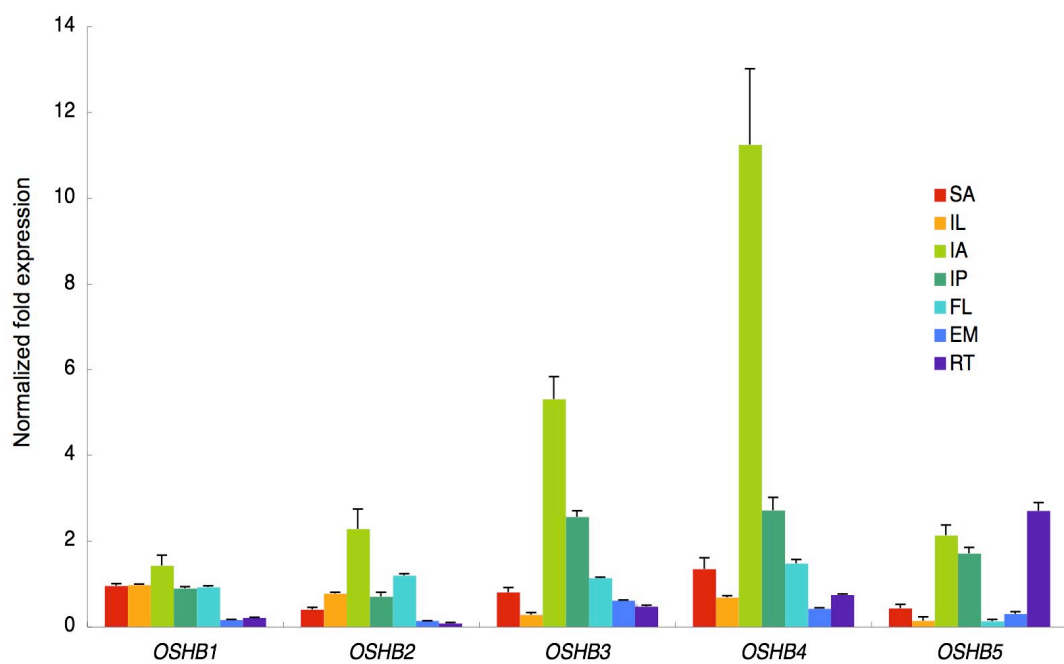
Figure S2. Real-time RT-PCR analysis of OSHB genes in various tissues. Expression level was normalized to that of eEF-1 \alpha . Bars indicate standard deviation. SA, shoot apex including young leaf primordia; IL, immature leaf; IA, 5-mm-long inflorescence apex; IP, 5-cm-long immature panicle; FL, immature flower; EM, embryos at 5 days after pollination; RT, root.
