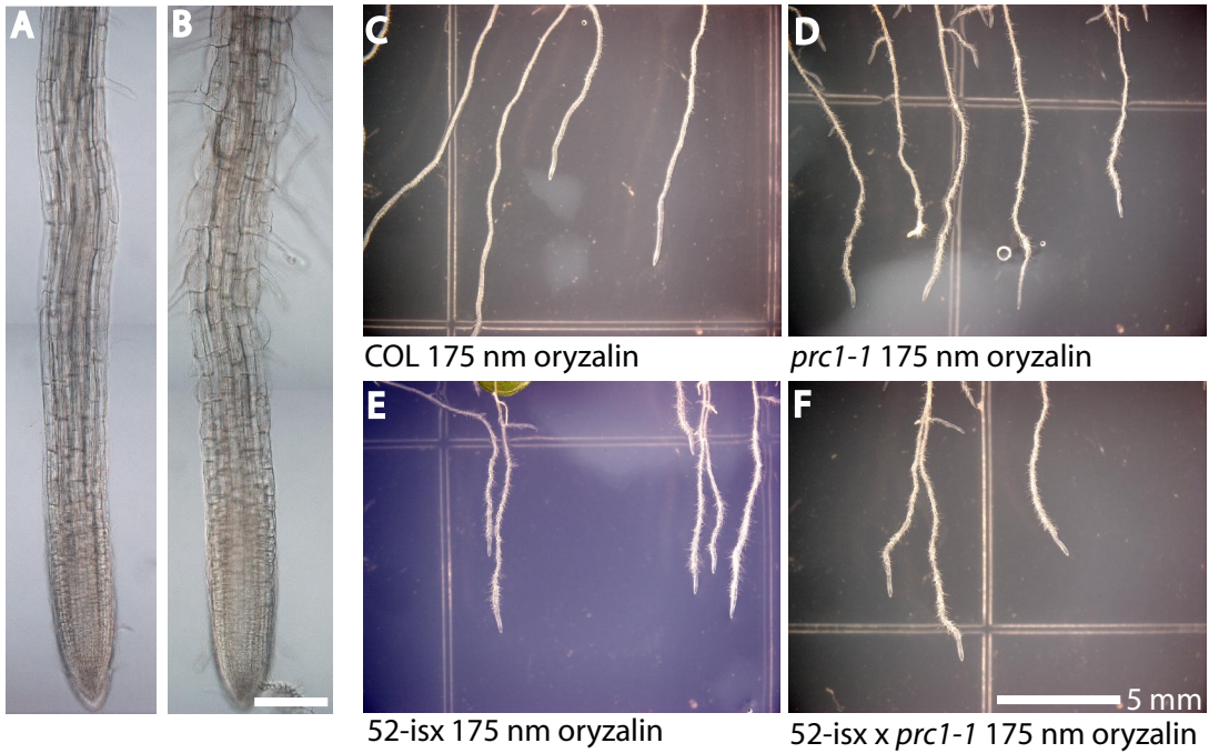
Figure S3. Mutant 52-isx carries an allele of prc1 . (A-F) Five day old light grown seedlings grown on 175 nM oryzalin. DIC image of COL (A) and 52-isx (B), note root swelling begins near the end of the elongation zone (before root hair emergence) but is more severe in fully differentiated trichoblast cells. Col (C) does not exhibit apparent swelling while prc1-1 (D) and 52-isx (E) have identical phenotypes. F1 seedlings from 52-isx x prc1-1 fail to complement indicating that the mutation in 52-isx is allelic to prc1-1 . Scale bar B=100 \mu m; F=5 mm.
