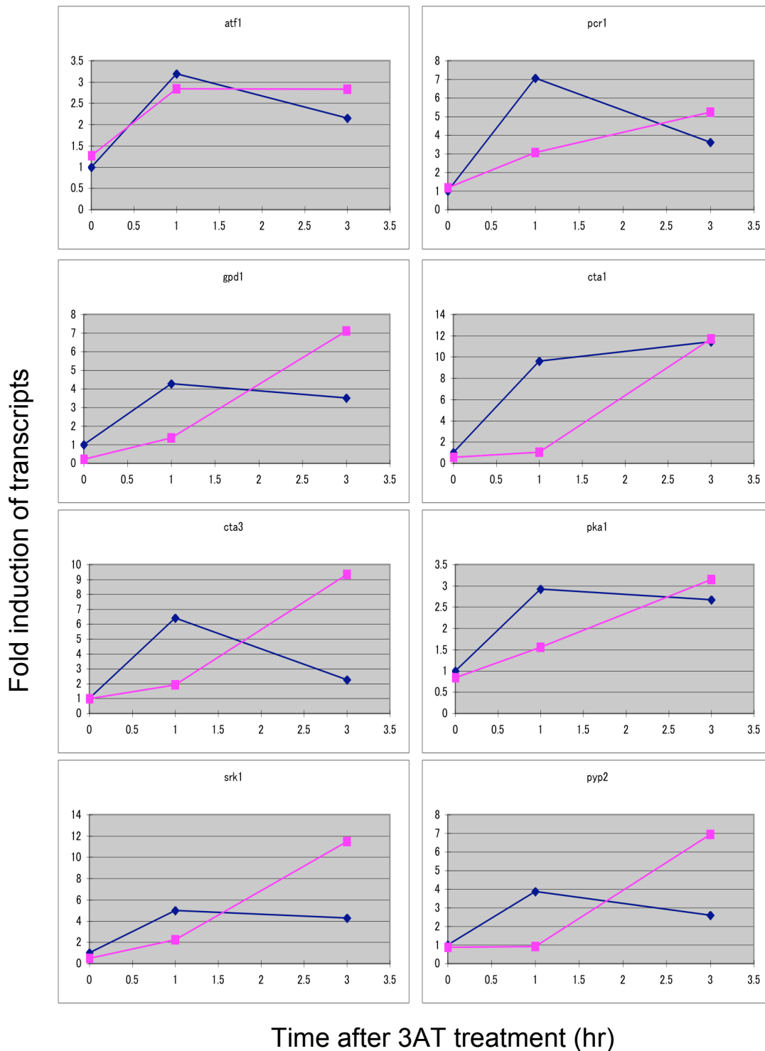
Fig. S1. 3AT-induced transcription profiles were plotted for selected cluster 2 (CESR) genes. Employed were microarray data from wild-type (purple) and int6Δ (pink) cells.
