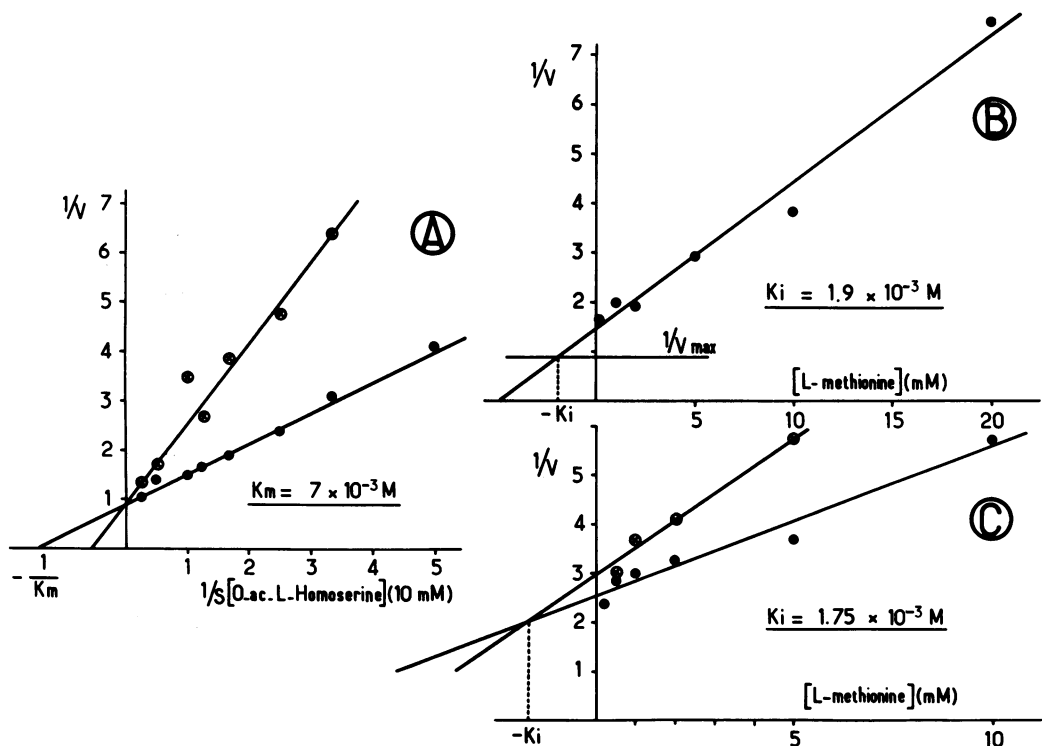
FIG. 2. Kinetic studies of homocysteine synthetase from S. cerevisiae . (A) Variation of activity with O -acetyl- L -homoserine concentration in the absence (●) or in the presence (⊗) of L -methionine 5 \times 10^{-3} \text{ M} [Lineweaver-Burk transformation (15)]. (B) Variation of activity ( 1/V ) with L -methionine concentration in the presence of O -acetyl- L -homoserine 10^{-3} \text{ M} . Same enzyme preparation was used for A and B. (C) Variation of activity ( 1/V ) with L -methionine concentration in the presence of O -acetyl- L -homoserine 4 \times 10^{-3} \text{ M} (●) and 8 \times 10^{-3} \text{ M} (⊗). K_i values have been calculated according to Dixon and Webb (4).
