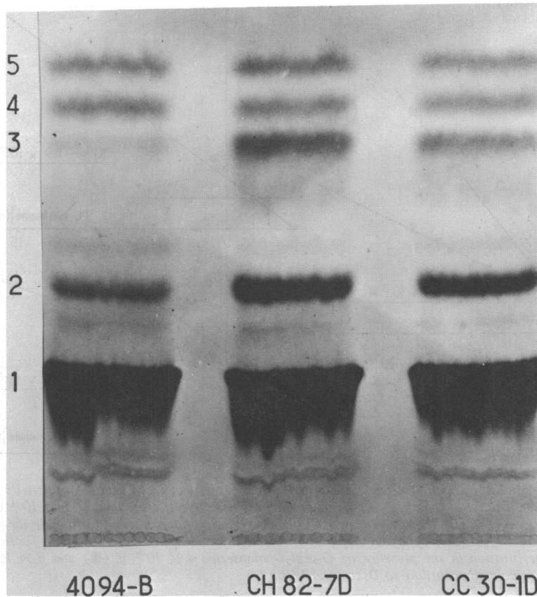
FIG. 1. Homoserine- O -transacetylase activity in different strains grown in a methionine-supplemented medium. Strains used are of the following genotypes: 4094-B: \alpha , ade_2 , ura_1 , eth_1^+ , eth_2^+ ; CH82-7D: \alpha , ade_2 , ura_1 , eth_1^+ , eth_2^+ ; CC30-1D: \alpha , ade_2 , ura_1 , eth_1^+ , eth_2^+ . Minimal medium was supplemented with DL-methionine 2 \times 10^{-3} M. Spot identification: 1, ^{14}\text{C} -4-DL-homoserine; 2, O -acetyl-DL-homoserine; 3, compound (ninhydrin-negative) derived from O -acetyl-homoserine; 4 and 5, radioactive impurities present in ^{14}\text{C} -4-labeled-DL-homoserine. The assay and solvent system have been described (25).
