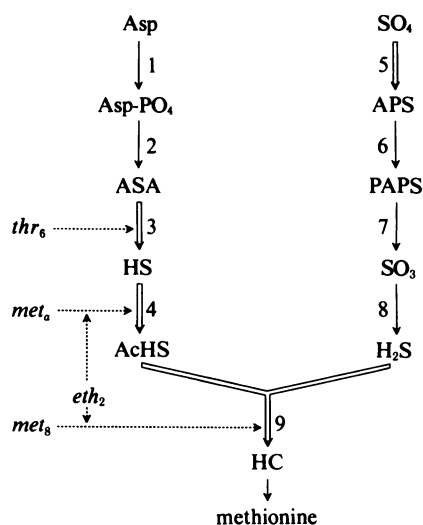
FIG. 3. Metabolic and regulatory scheme for methionine biosynthesis in S. cerevisiae . Step numbers correspond to the following enzymes: 1, aspartate kinase ( L -aspartate 4-phosphotransferase; EC 2.7.2.4). 2, ASA dehydrogenase [ L -aspartate- \beta -semialdehyde: NADP oxidoreductase (phosphorylating); EC 1.2.1.11]. 3, HS-dehydrogenase ( L -homoserine: NAD oxidoreductase; EC 1.1.1.3). 4, L -Homoserine- O -transacetylase (Nagai and Flavin, 20). 5, ATP-sulfurylase (ATP: sulfate adenylate transferase; EC 2.7.7.4). 6, APS-kinase (ATP: adenylylsulfate-3'-phosphotransferase; EC 2.7.1.25). 7, PAPS-reductase (Pasternak et al., 21). 8, Sulfite reductase (hydrogen sulphide: NADP oxidoreductase; EC 1.8.1.2). 9, Homocysteine synthetase (Wiebers and Garner, 38). Relevant structural genes are connected to reactions by broken arrows. Compounds are abbreviated as in the scheme given in the introduction. Large empty arrows indicate enzymatic steps repressed by methionine.
