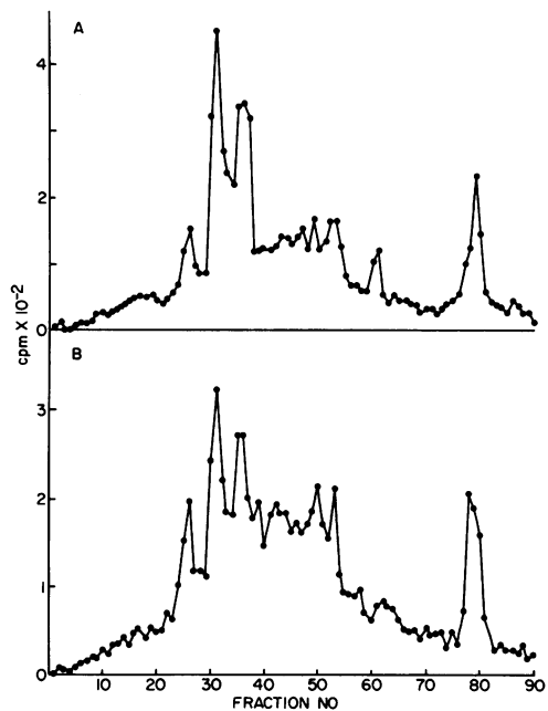
FIG. 1. Distribution of radioactivity in the soluble polypeptides synthesized during the first hour of germination of B. theobromae spores. One liter of the spore suspension was pulsed from 0 to 1 hr with 100 \mu Ci of a mixture of 12 3 H-amino acids. The spore suspension was harvested and divided into two equal samples. One sample was immediately frozen (A), and the other was returned to fresh medium containing 12 unlabeled amino acids (each at 0.002 M) and incubated an additional 4 hr before harvesting (B). The soluble protein fraction was isolated and electrophoresed as described in the text.
