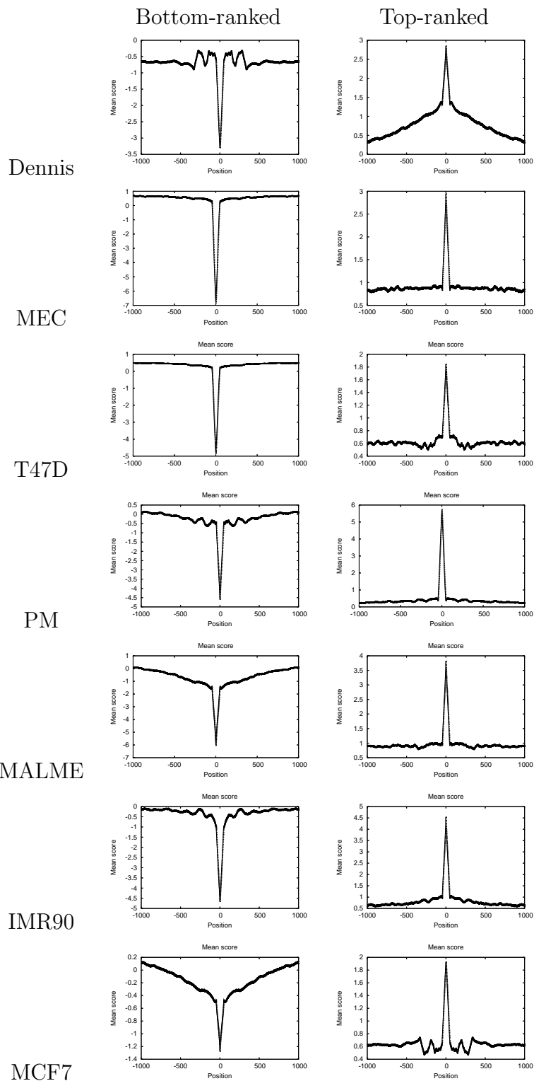
Figure S1: This figure is similar to Figure 5, but the panels were generated using top- and bottom-scoring probes from each of the SVMs.
