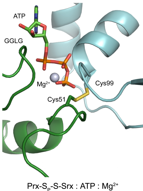
Figure S1. Crystal structure of Srx:ATP:Mg 2+ modeled onto the disulfide-bonded Srx-PrxI crystal structure (PDB # 2RII).
