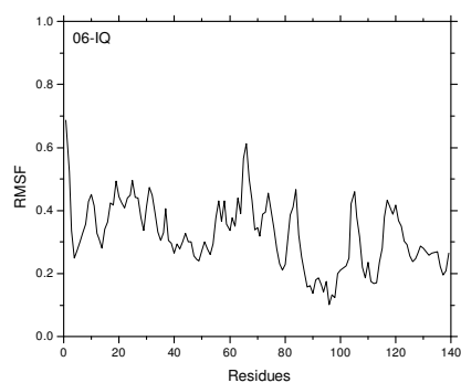
Figure S5. Structural fluctuations. Molecular dynamics of the NMR-derived conformations with the ligands. The Root mean square fluctuations (RMSF's, in Å) are reported for the 26 stable complexes.
