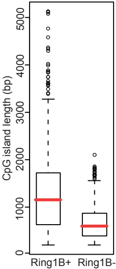
Figure S9. Length of CpG islands in Ring1B-positive and Ring1B-negative bivalent promoters.
