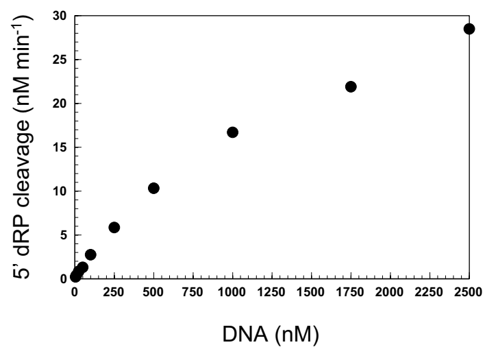
Fig. S1. Initial rates of 5' dRP cleavage.
