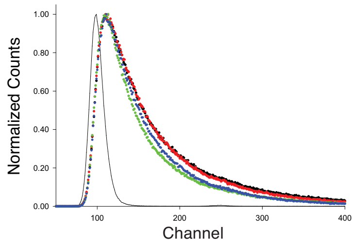
Figure 2: Time resolved decays of Trp12 in TnC(12W/C51±AEDANS) showing the effect of TnI addition (48.8 ps/channel). TnC in 160 \mu\text{M} \text{Ca}^{2+} : donor-only (black), donor-acceptor (green). TnC in 160 \mu\text{M} \text{Ca}^{2+} + 2-fold excess of TnI: donor-only (red). Donor-acceptor (blue). Impulse response (black line).
