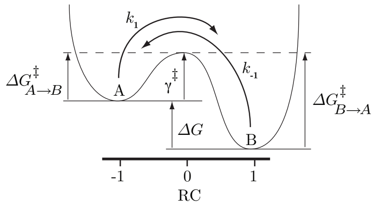
Figure 1: Energy surface of a reversible noise-induced transition in a bi-metastable potential.
