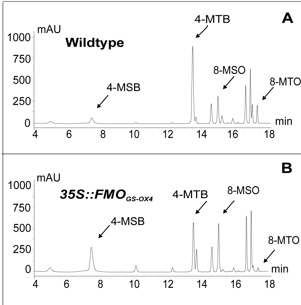
Supplemental Figure S2. Glucosinolate (GSL) profile of seed in T1 generation of 35S::FMO_{GS-OX4} and wild-type plant. A: wild-type plant; B: 35S::FMO_{GS-OX4} line1; Abbreviations: 4-MTB, 4-methylthiobutyl GSL; 4-MSB, 4-methylsulfinylbutyl GSL; 8-MTO, 8-methylthiooctyl GSL; 8-MSO, 8-methylsulfinyl-octyl GSL.
