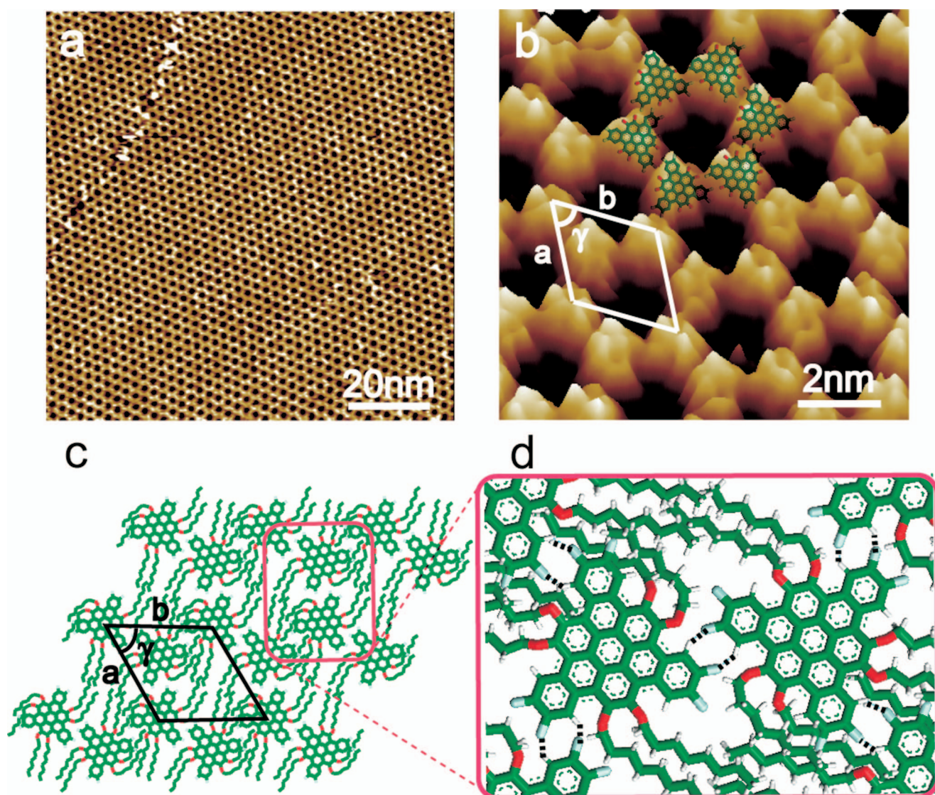
Fig. S1. Self-assembly of FTBC-C8 on HOPG. (a) Large-scale STM image. V_{\text{bias}} = -1.32 V; I_t = 120 pA. (b) High-resolution STM image. V_{\text{bias}} = -1.53 V; I_t = 529 pA. (c) Proposed structural model for the ordered adlayer. (d) Possible hydrogen bonds between the molecules indicated by black dashed lines.
